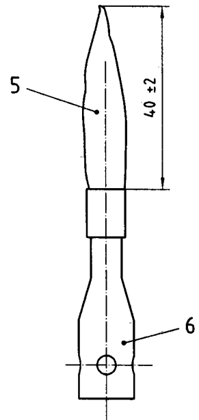
c) Vertical flame height
